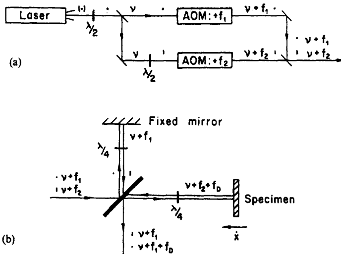
Fig. 1. Optical arrangements for Doppler interferometer: (a) beam formation (·, vertical; |, horizontal polarization); (b) beam paths.
